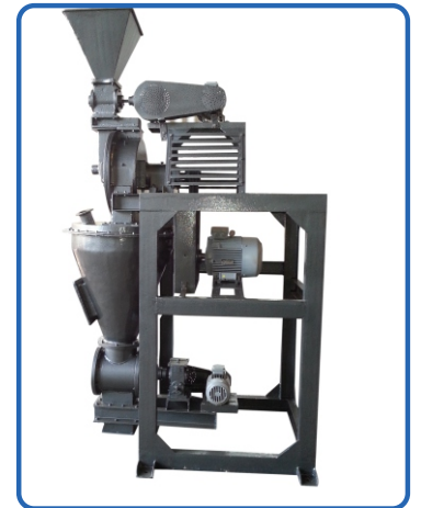
Micro Pulverizer with Auto Feeding and Auto Discharge
